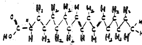
LINOLEIC ACID
