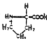
PROLINE
