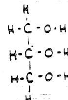
GLYCEROL
