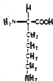
LYSINE
