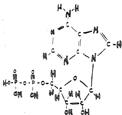
ADENOSINE DIPHOSPHATE
