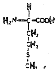
METHIONINE
