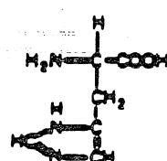
HISTIDINE
