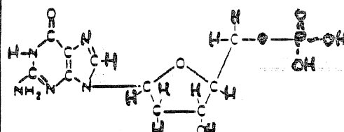
DEOXYRIBOSE GUANINE
