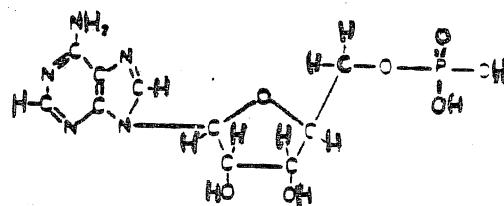
RIBOSE ADENINE
