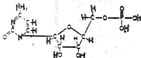
RIBOSE CYTOSINE
