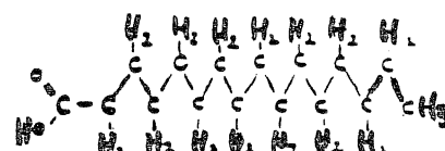
PALMITIC ACID
