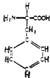
PHENYLALANINE
