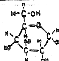
GLUCOSE
