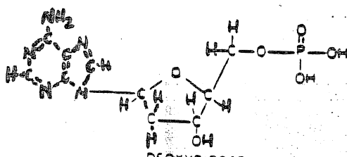
DEOXYRIBOSE ADENINE
