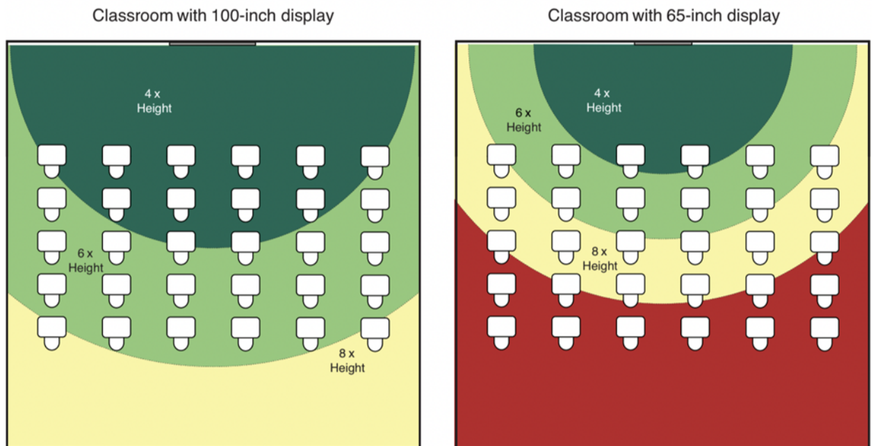
Typical 952 Square Foot Classroom with 30 Desks (30.85 feet W x 30.85 feet D)
